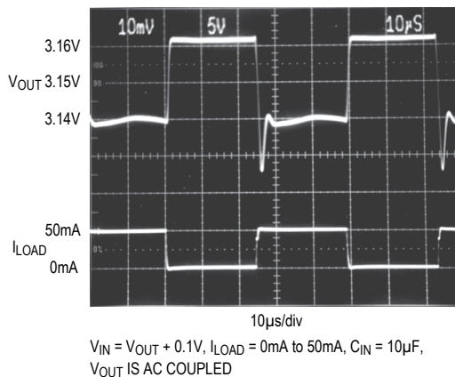
LOAD TRANSIENT
