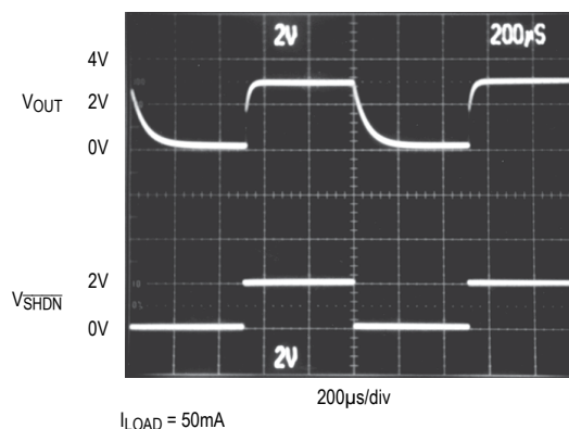
MAX8864 SHUTDOWN
